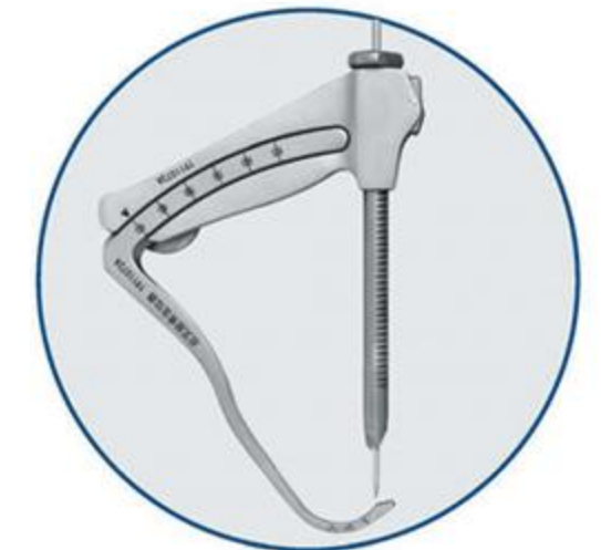
后叉胫骨定位器+定位器+钻套 Posterior fork tibial alignment hook+ positioner + drill sleeve
