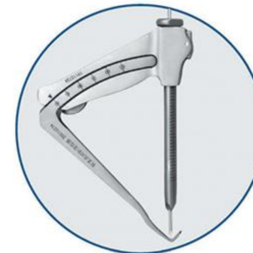
前叉点对点定位器+定位器+钻套 Front fork point-to-point locator+ positioner + drill sleeve
